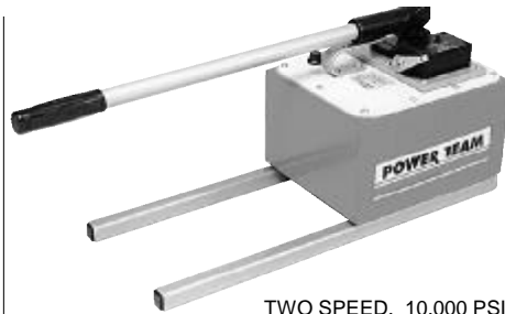
LARGE VOLUME HAND PUMPS
